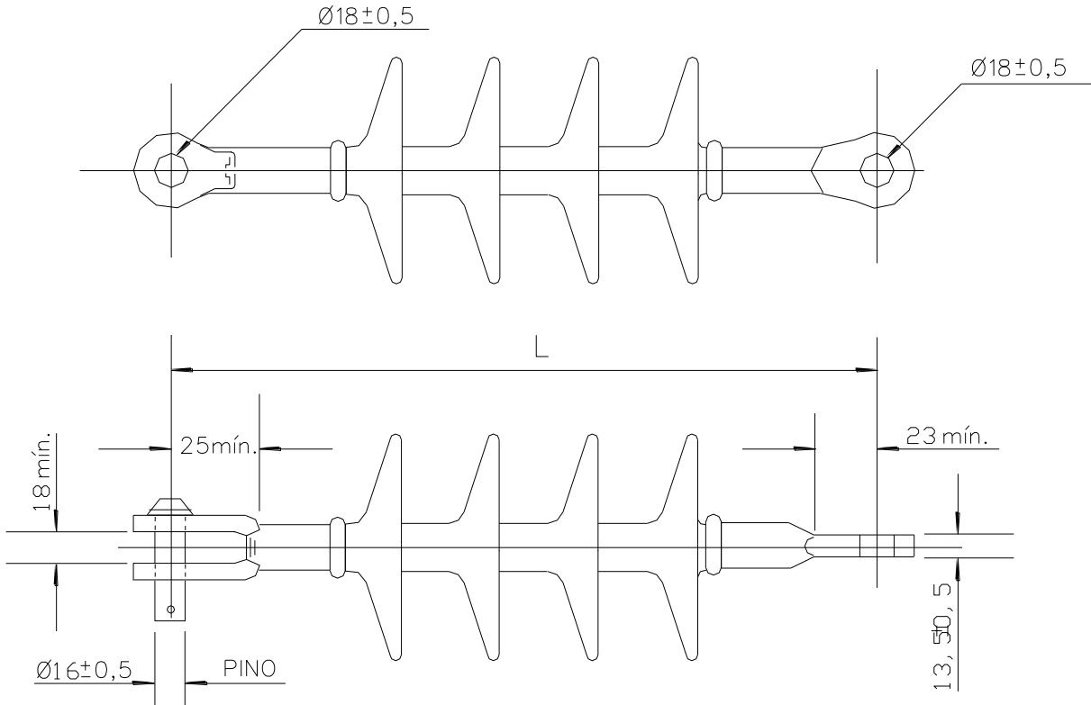
PINO
